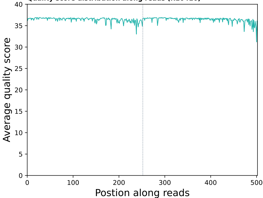
Quality score distribution along reads (R10416)
